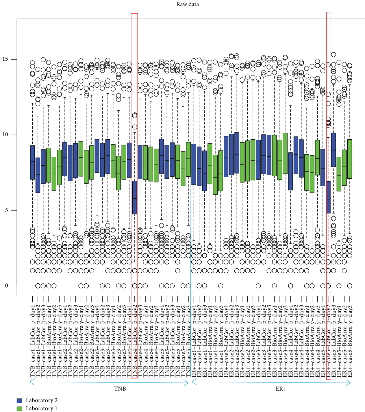
FIGURE 1: Boxplot analysis of the 60 replicate samples from NanoString experiment, with 5 unique TNB samples and 5 ER+ samples, prepared by two different labs and 3 different days. TNB: triple-negative breast cancer samples; ER+: estrogen receptor-positive breast cancer samples. The red lines show the outliers.
